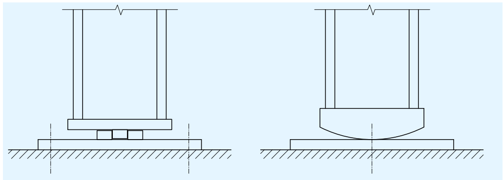
Figure 3.10 Examples of zero stiffness column bases
